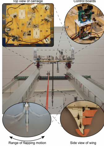
Figure 3: Carriage setup highlighting the pulley system setup, control boards, range of wing motion and wing structure.
